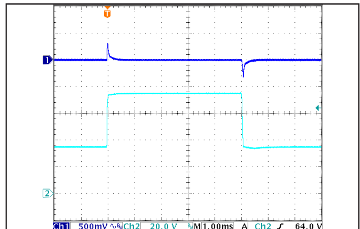
Figure 6: Output voltage response to step-change in input voltage (250 V/ms). Load cap: 100 μF, electrolytic output capacitance. Ch 1: V out (500 mV/div), Ch 2: V in (20 V/div).
