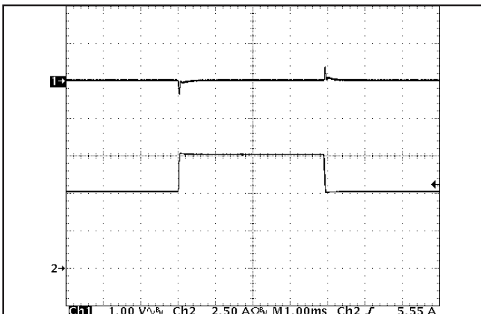
Figure 5: Output voltage response to step-change in load current (66% -100% - 66% of I out (max); dI/dt = 0.2 A/μs). Load cap: 1 μF ceramic and 15 μF tantalum capacitors. Ch 1: V out (1 V/div), Ch 2: I out (2.5 A/div).
