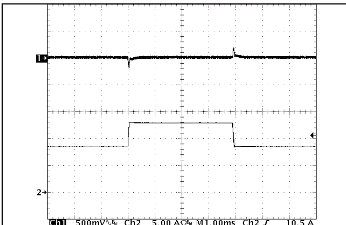
Figure 5: Output voltage response to step-change in load current (66% -100% - 66% of I out (max); dI/dt = 0.2 A/μs). Load cap: 1 μF ceramic and 15 μF tantalum capacitors. Ch 1: V out (500 mV/div), Ch 2: I out (5 A/div).
