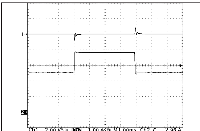
Figure 5: Output voltage response to step-change in load current (66% -100% - 66% of I out (max); dI/dt = 0.2 A/μs). Load cap: 1 μF ceramic and 15 μF tantalum capacitors. Ch 1: V out (2 V/div), Ch 2: I out (1 A/div).
