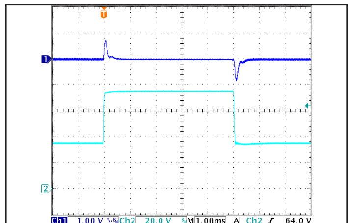
Figure 6: Output voltage response to step-change in input voltage (250 V/ms). Load cap: 100 μF, electrolytic output capacitance. Ch 1: V out (1 V/div), Ch 2: V in (20 V/div).
